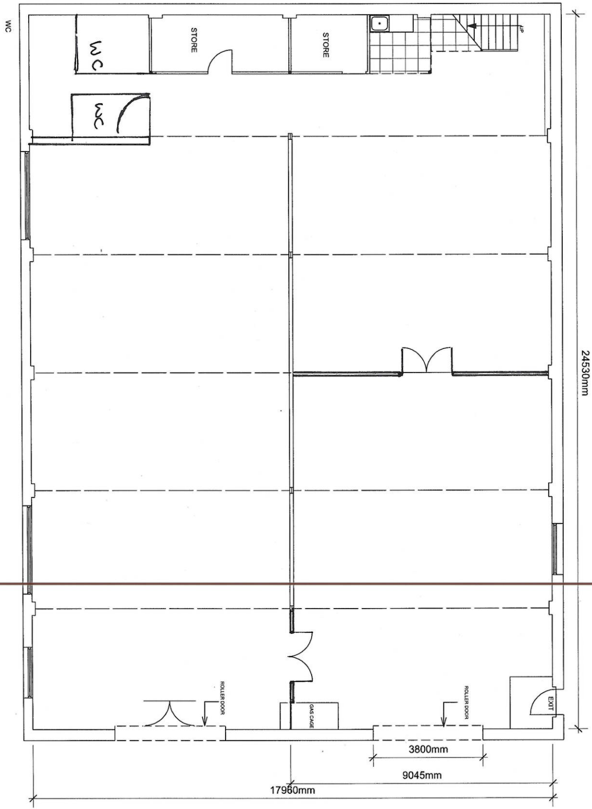
PLAN
