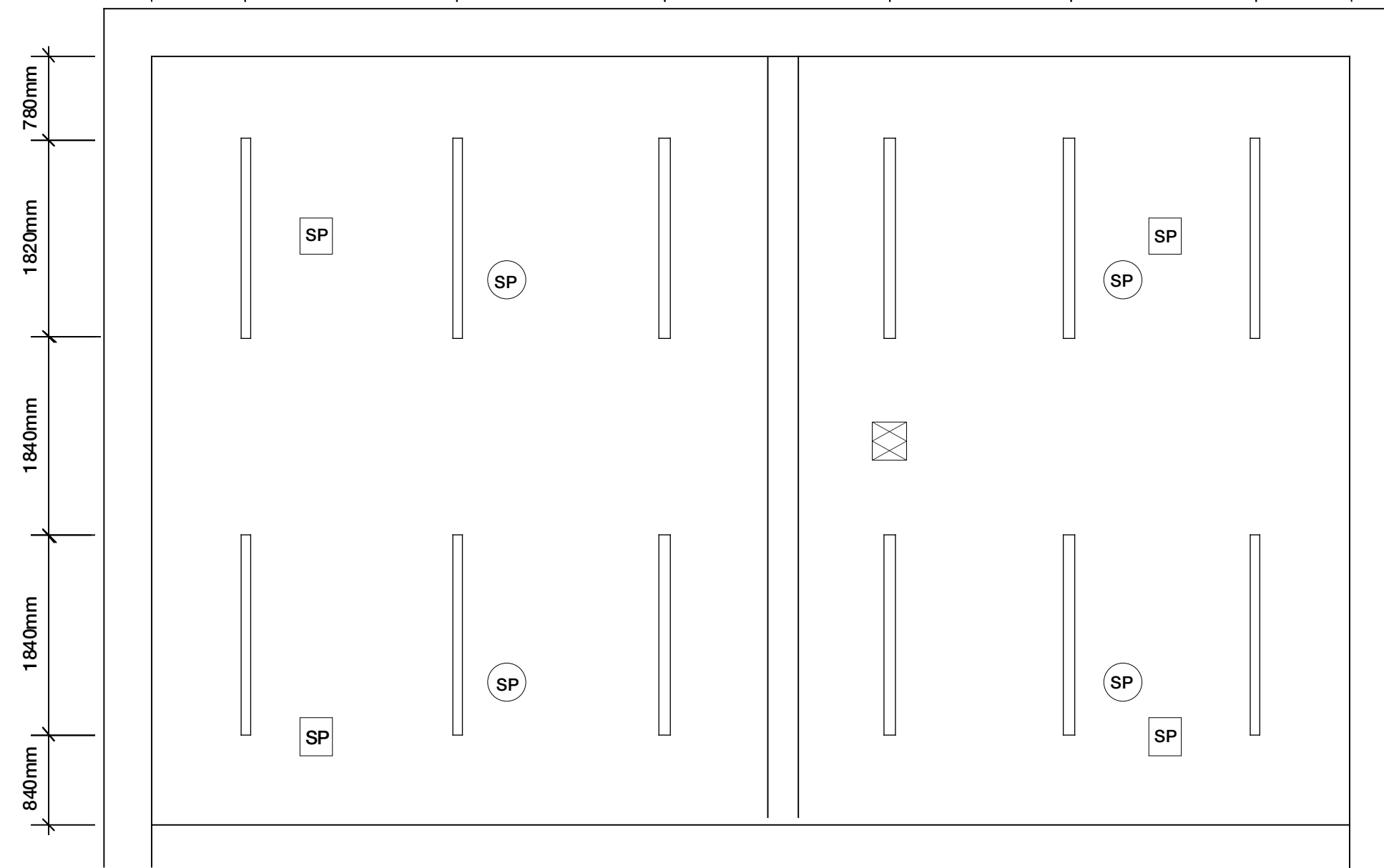
REFLECTED CEILING PLAN (RCP)
