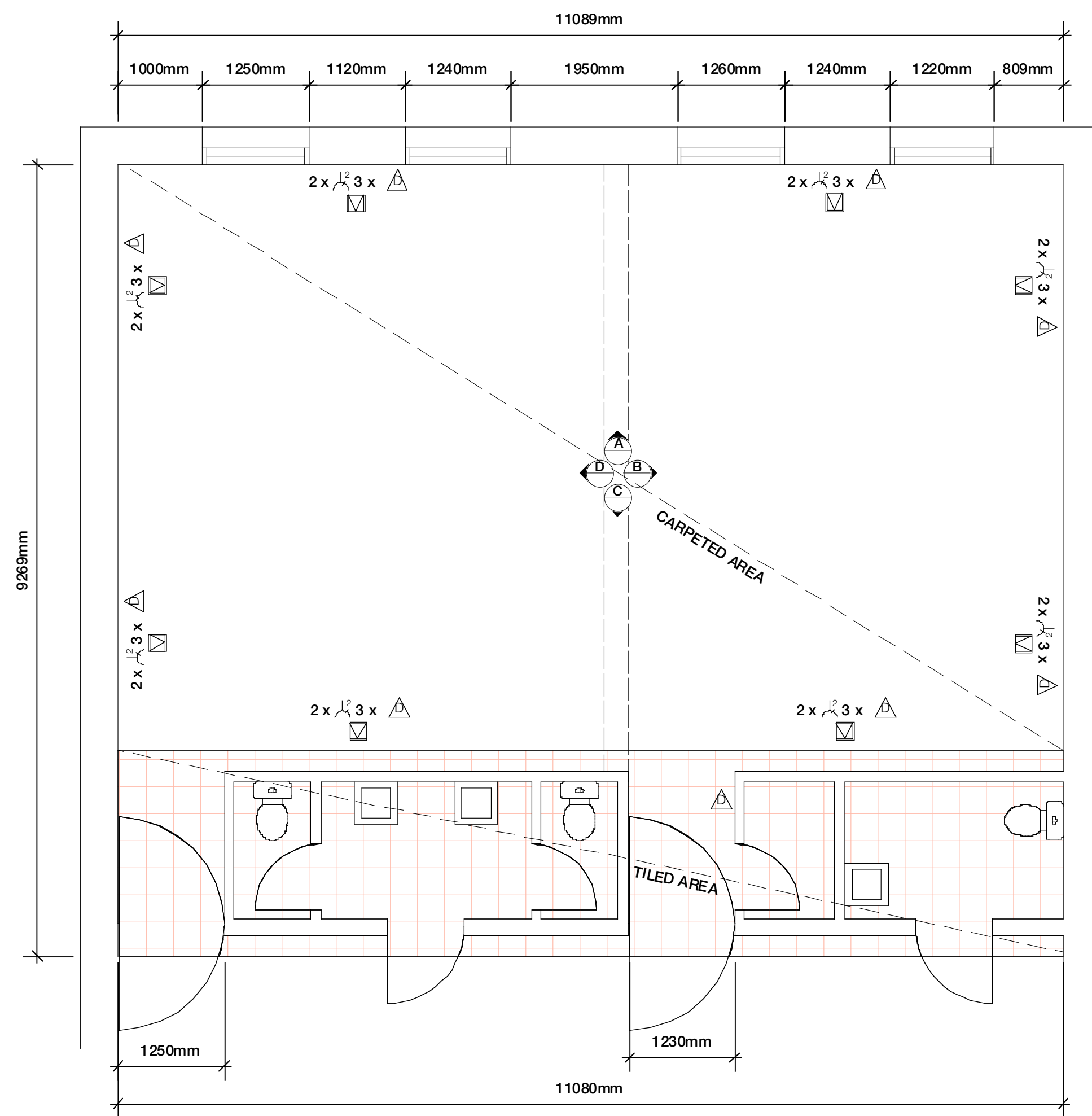
PLAN
